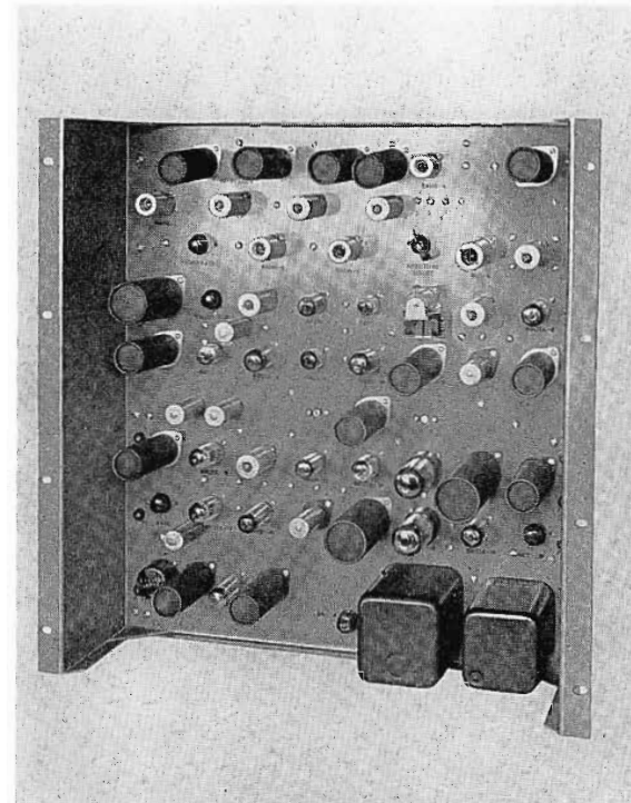
FIG. 6. The Vidicon Processing Amplifier.
