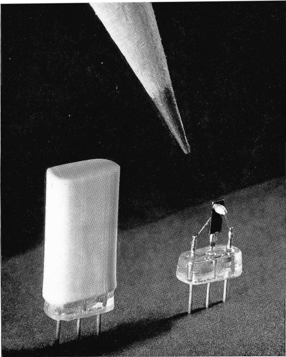
FIG. 20. At right, pencil points to developmental junction-type transistor before embedment in plastic container. At left, the sealed unit.
