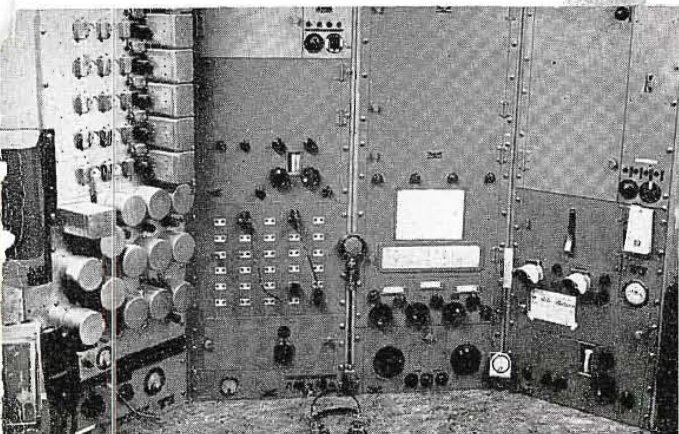
RCA Communications frequency measuring installation
