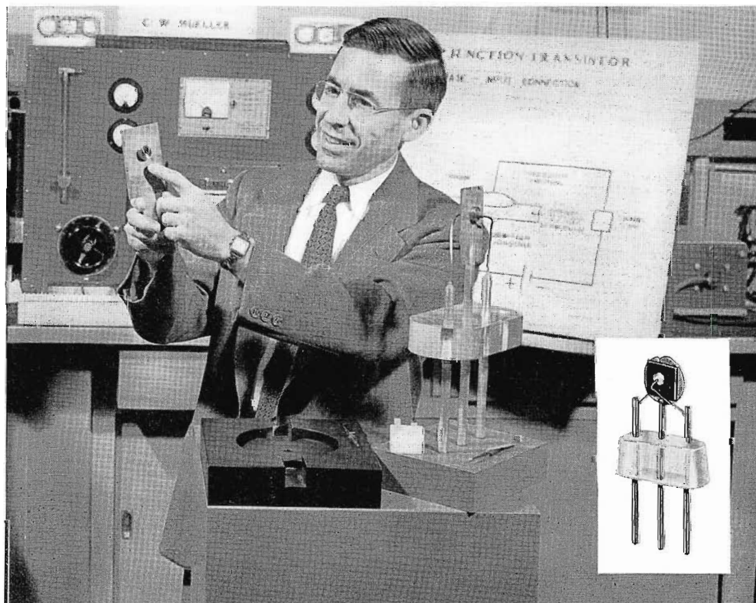
FIG. 24. Dr. C. W. Mueller of the research staff of the David Sarnoff Research Center of RCA Princeton, N. J., points to a "blown-up" model of the heart of an RCA developmental junction-type transistor. Complete interior model is seen at right. A "p-n-p" junction-type transistor is shown in the inset at lower right.
