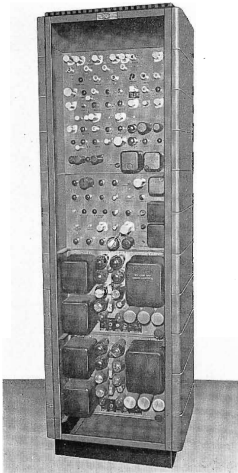
FIG. 8. View of the Vidicon power supplies and amplifier units which are rack mounted for convenience.
