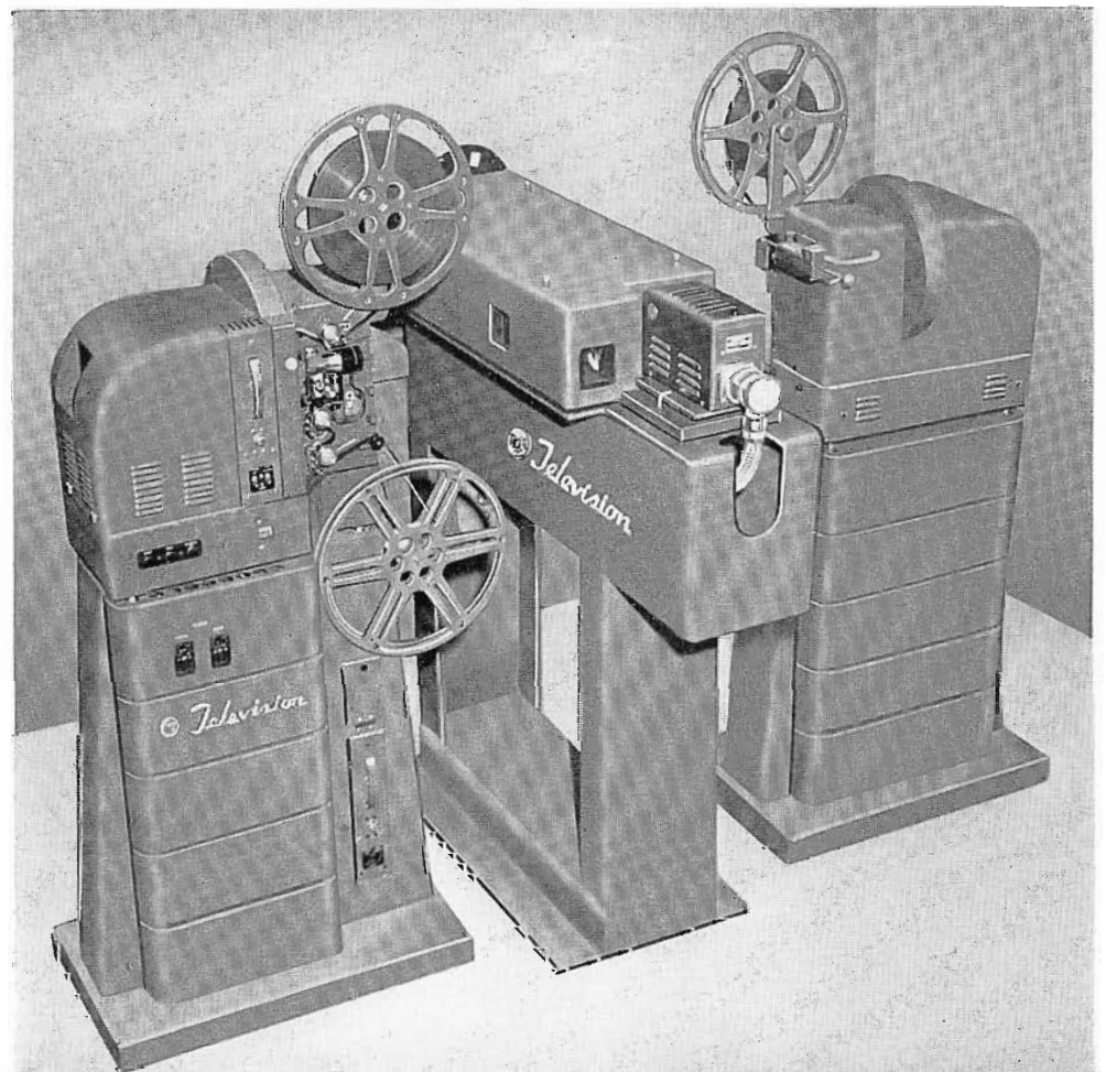
FIG. 2. The Vidicon Film Camera shown in multiplexed use. Here two TP-16 Projectors and a 35mm Slide Projector are directed into the Vidicon Multiplexer (center).
