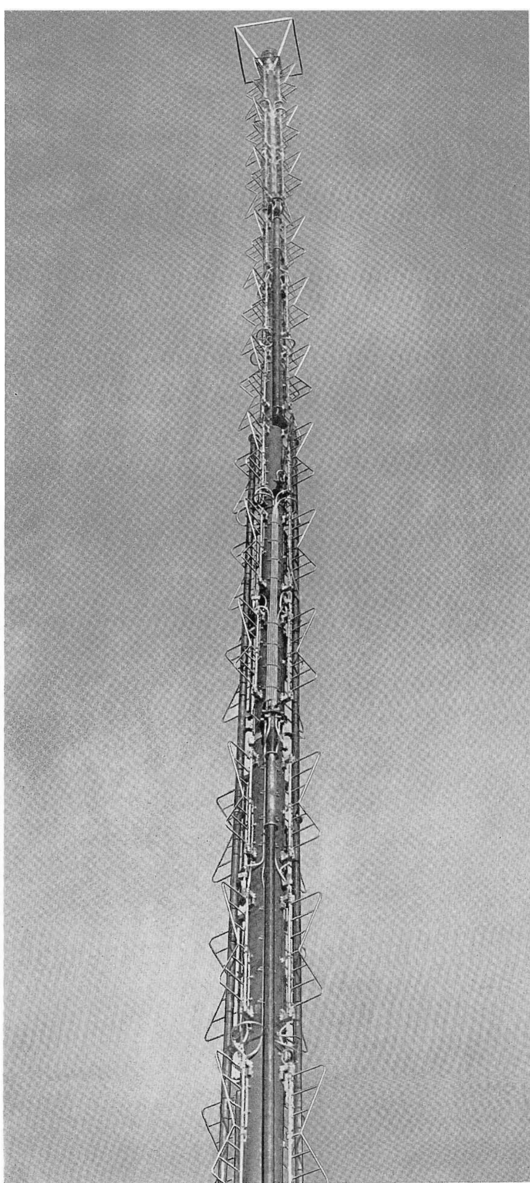
FIG. 2. Closeup view of the 12-section Superturnstile as it appears when installed in normal upright position. The new 12-section (with a gain of 9 approximately) retains all of the inherent features of previous Superturnstile plus the desirable feature of much improved close-in coverage.
