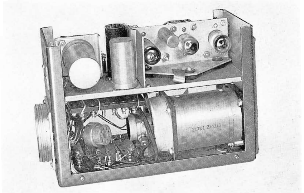
FIG. 4. Closeup of the Vidicon Camera with cover removed to illustrate mechanical details.
