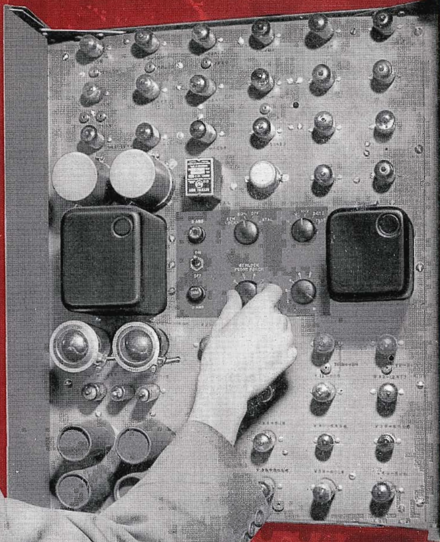
New RCA single-unit Sync Generator takes less than one-third the rack space needed by other sync systems
