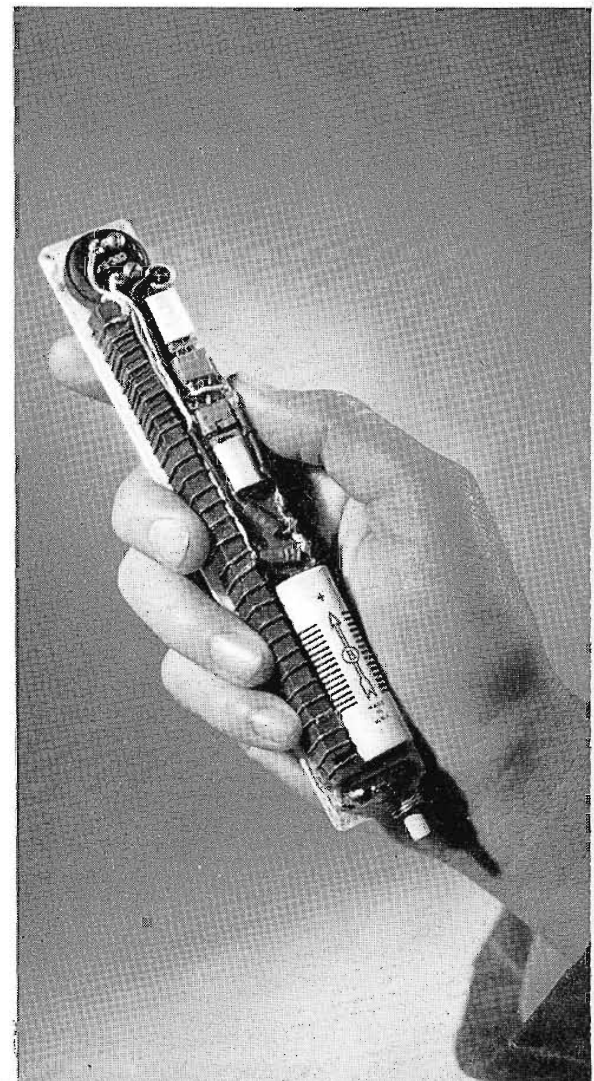
FIG. 7. A cigar-size experimental microphone-transmitter, modulated by a tiny built-in dynamic microphone. Employs two developmental junction type transistors, coil and battery.
