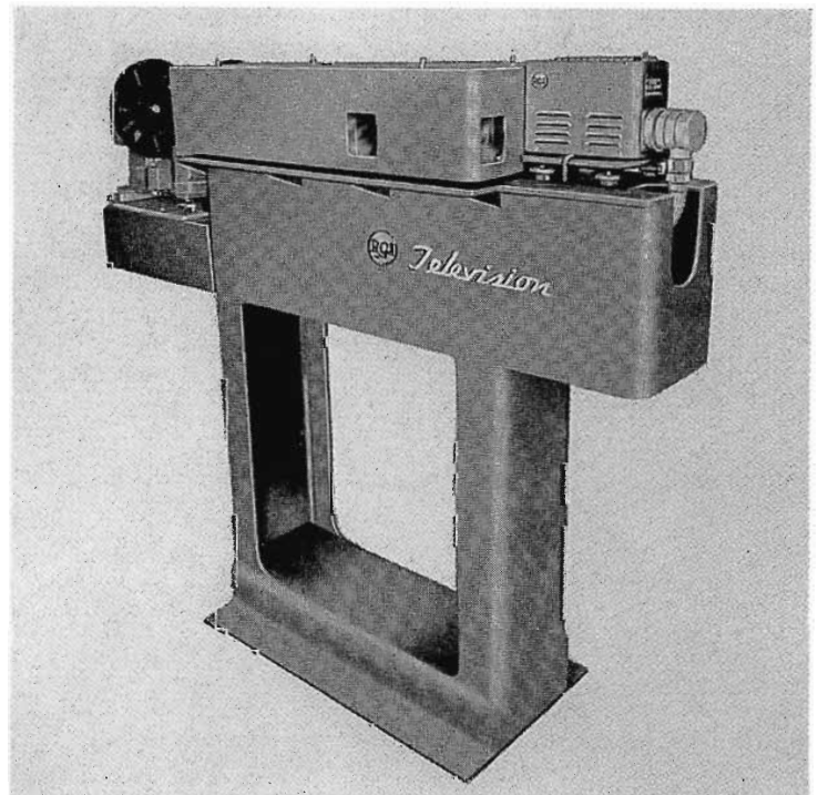
FIG. 11. The Vidicon Multiplexer, TP-11A, has been designed especially for use with the Vidicon Film Camera. This unit will accommodate two 16mm or 35mm film projectors, a 35mm slide projector and a Telop slide and opaque projector.
