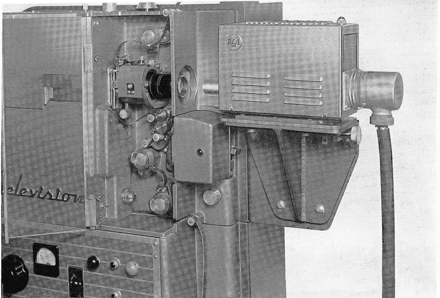
FIG. 1. View of the Vidicon Film Camera shown coupled to an RCA TP-6A Professional 16mm Television Projector.
