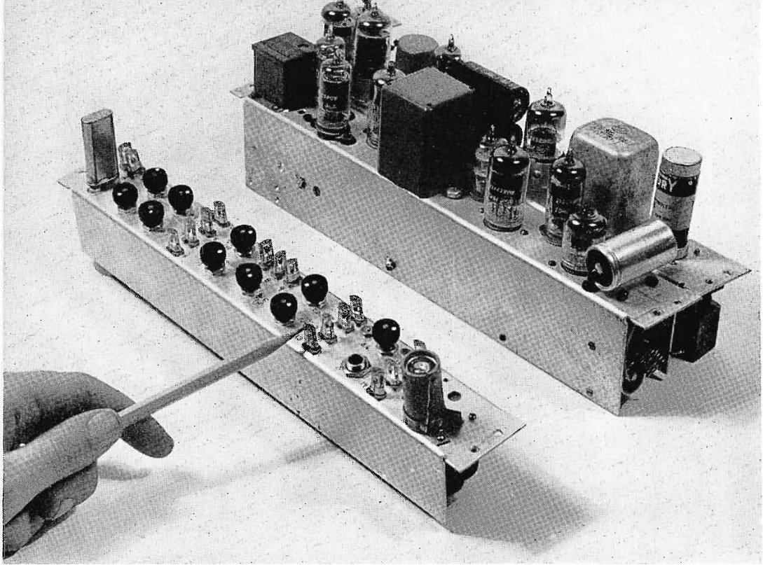
FIG. 6. In the foreground, a unit of an experimental "Walkie-Lookie" in comparison with a corresponding tube-equipped unit which was used in earlier experiments. Seventeen point-contact transistors perform the function of twenty-two tubes.
