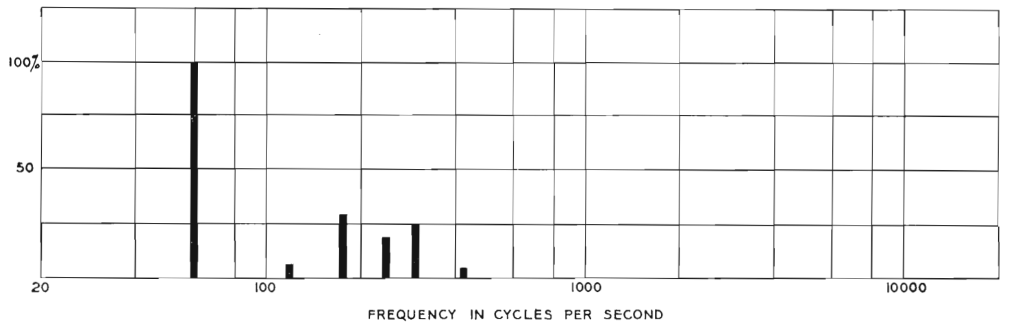
FIG. 6. Field analysis near 80-watt fluorescent fixture.
