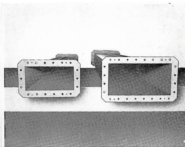
FIG. 6. End view of Waveguide Rigid Sections. Cross-section of WR-1150 (left) is 5\frac{3}{4}'' \times 11\frac{1}{2}'' —18 holes in flanges. Cross-section of WR-1500 is 7\frac{1}{2}'' \times 15'' —24 holes in flanges.
