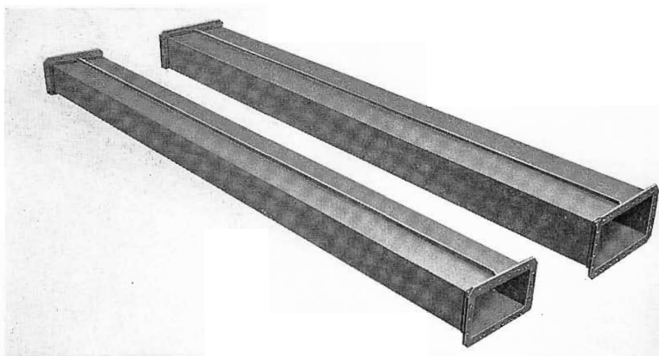
FIG. 5. Ten-foot Waveguide Rigid Sections, Type WR-1150 and Type WR-1500 placed side-by-side to demonstrate their comparative physical size. Type WR-1150 (in foreground) is MI-27311-1. Type WR-1500 is MI-27310-1.
