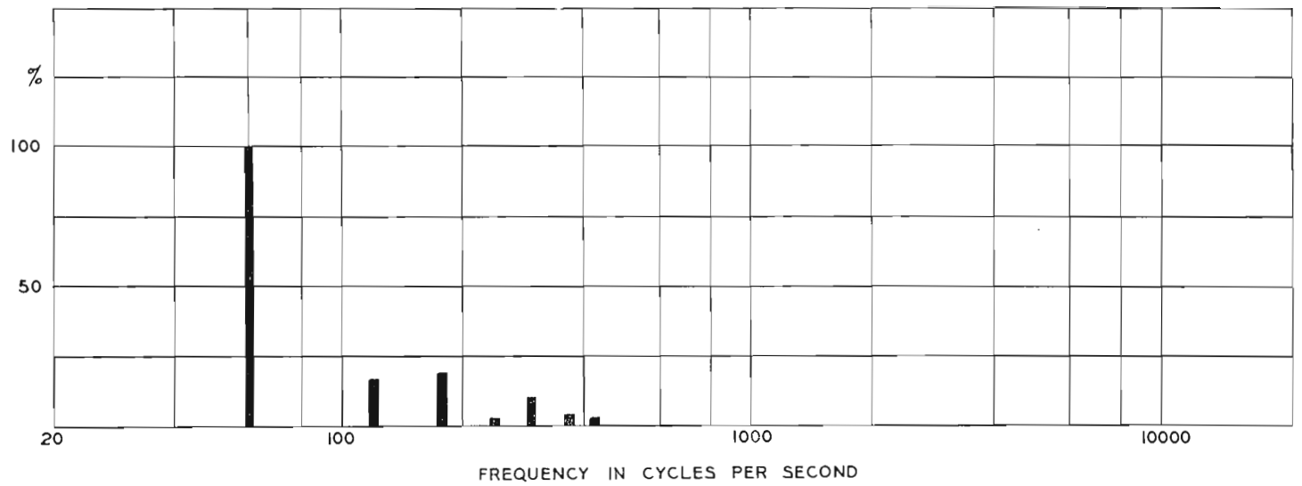
FIG. 4. Field analysis in a typical Broadcast studio.
