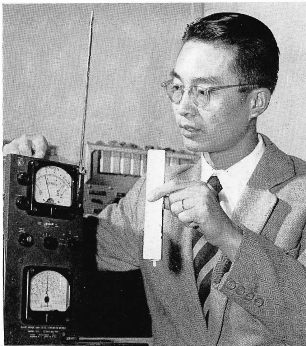
FIG. 9. The cigar-size experimental microphone-transmitter, made to explore possibilities of a low-cost wireless microphone-transmitter. Effective within radius of 25 feet.
