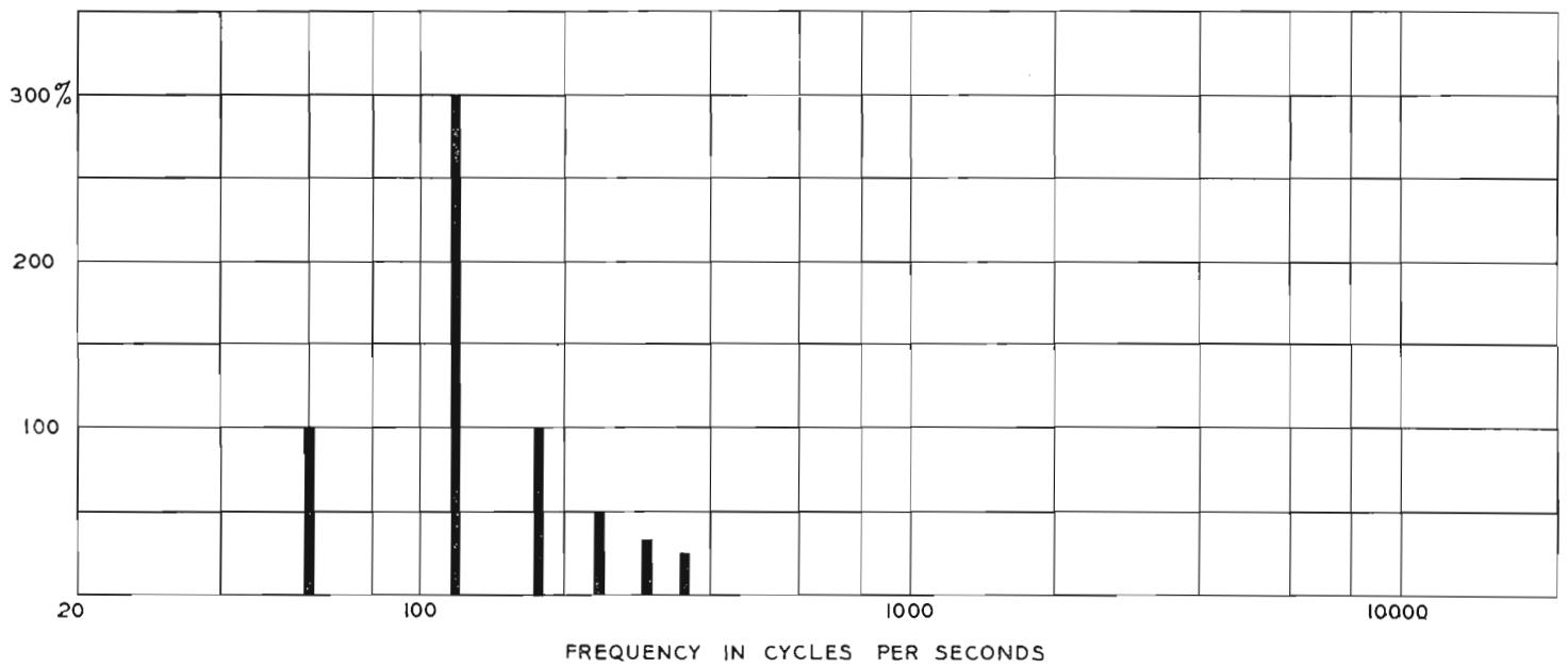
FIG. 5. Field analysis near power amplifier.
